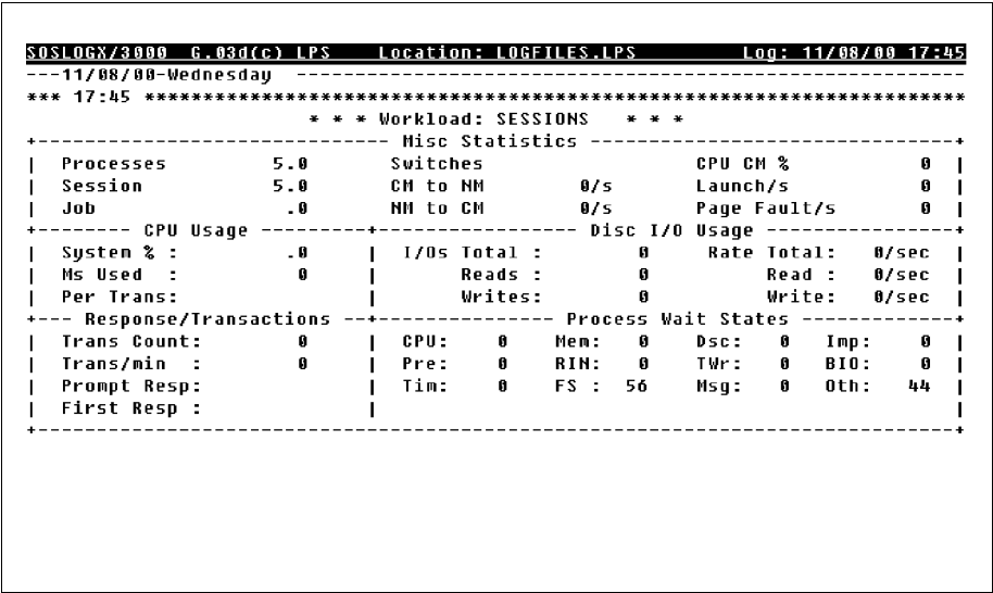
Figure 27.11 SOSLOGX SESSIONS Workload Detail report
