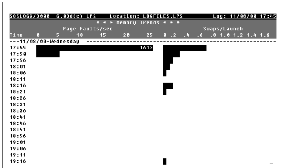
Figure 27.2 SOSLOGX Memory Trends screen
