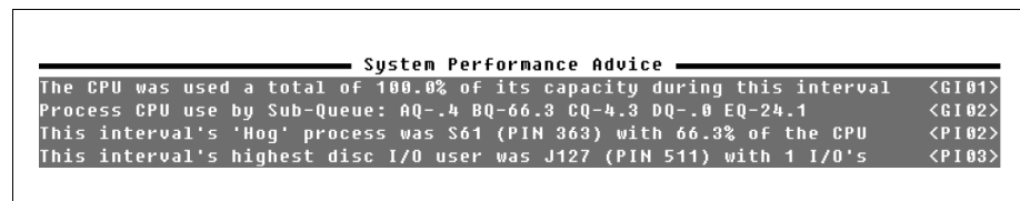
Figure 6.4 SOS Global Summary screen: System Performance Advice messages
